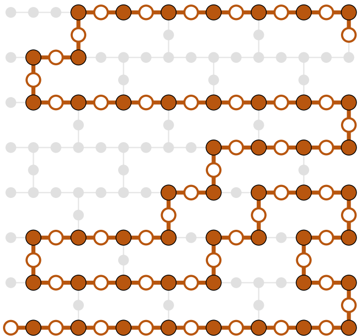
circuit 4: 1 instances, 99 qubits
