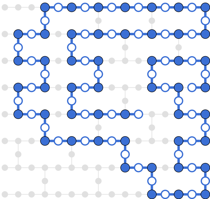
circuit 5: 1 instances, 99 qubits
