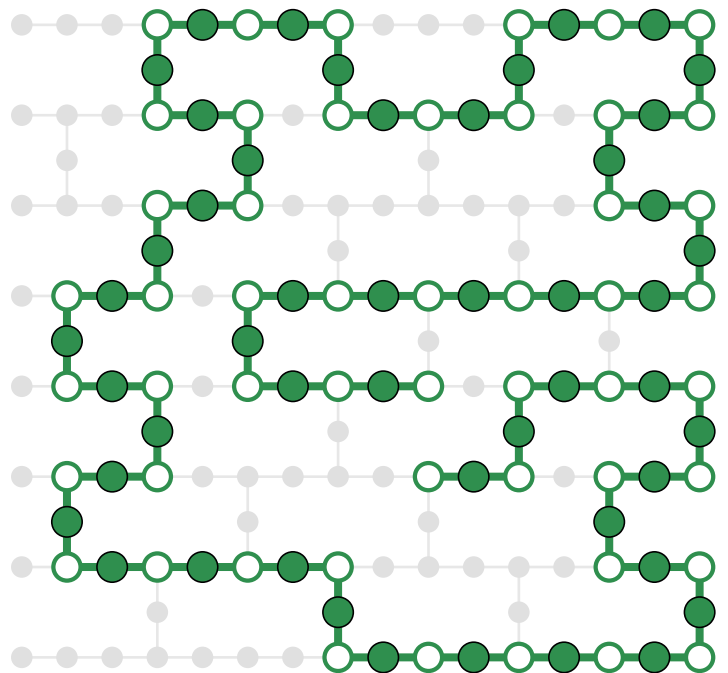
circuit 6: 1 instances, 99 qubits
