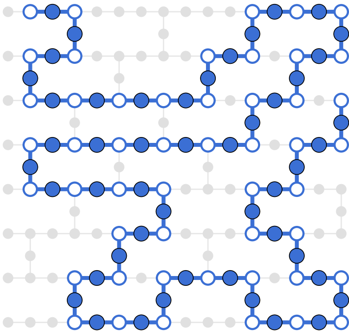
circuit 1: 1 instances, 99 qubits
