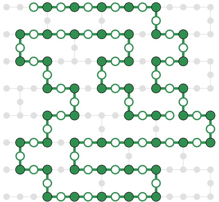
circuit 2: 1 instances, 99 qubits
