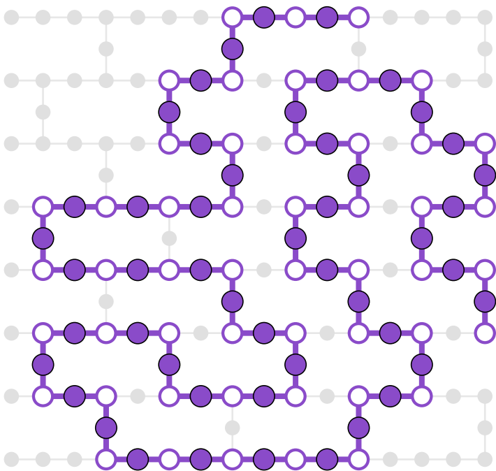
circuit 3: 1 instances, 99 qubits
