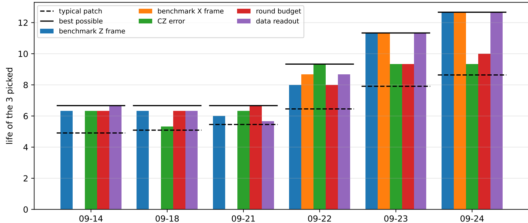
picking 3 patches
