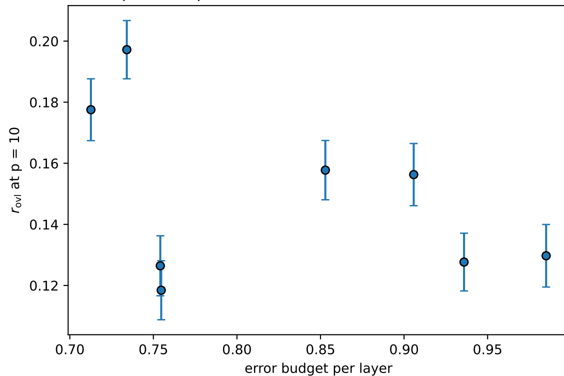
p = 10 : Spearman rho = -0.38 ( P = 0.352 , n = 8 )
