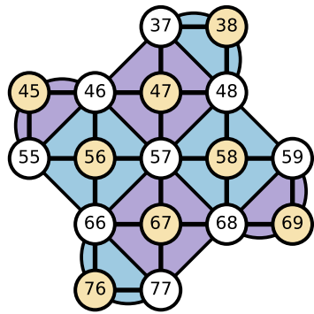
shaded, in the colours of the checks: the ground covered by the scanned placements, 11 at d = 3 , 8 at d = 5
