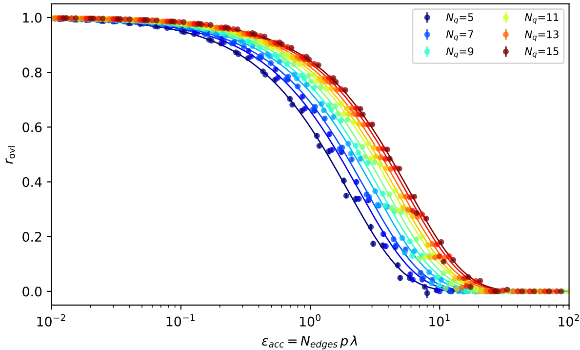
approximation-ratio overlap, all depths
