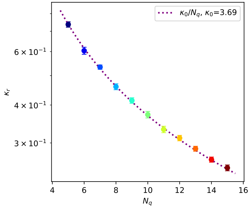
\kappa_r against chain length
