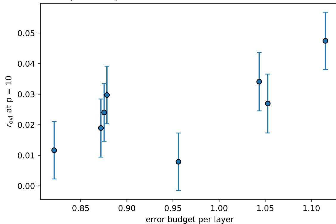
p = 10 : Spearman rho = +0.67 ( P = 0.071 , n = 8 )
