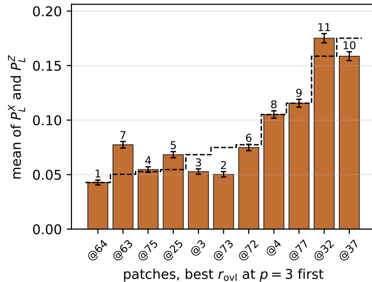
sorted by the X frame: \rho = 0.77 , mean shift 1.5
