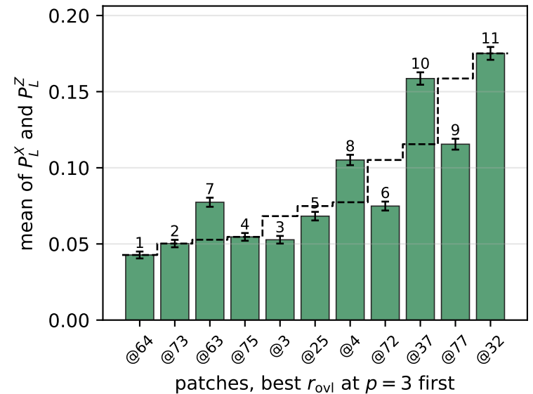
sorted by the XZ frame: \rho = 0.87 , mean shift 1.1
