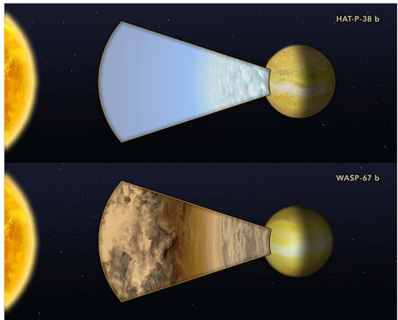
Clear versus cloudy atmospheres on two exoplanets. [179]
