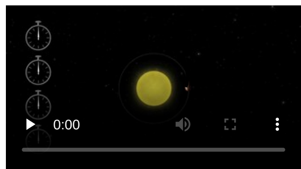
Animation showing difference between planet transit timing of one-planet and two-planet systems
