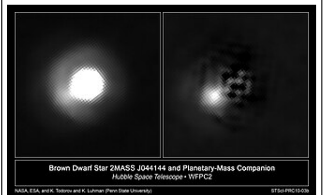
2MASS J044144 is a brown dwarf with a companion about 5–10 times the mass of Jupiter. It is not clear whether this companion object is a sub-brown dwarf or a planet.
