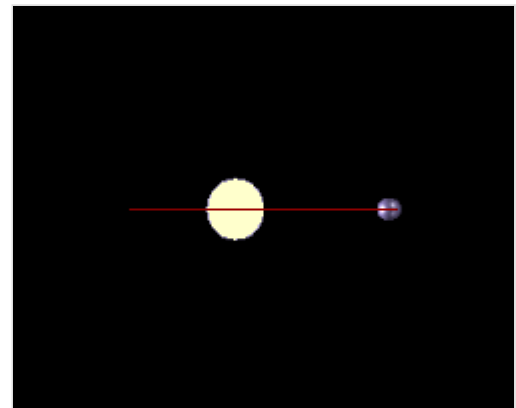
When the star is behind a planet, its brightness will seem to dim
