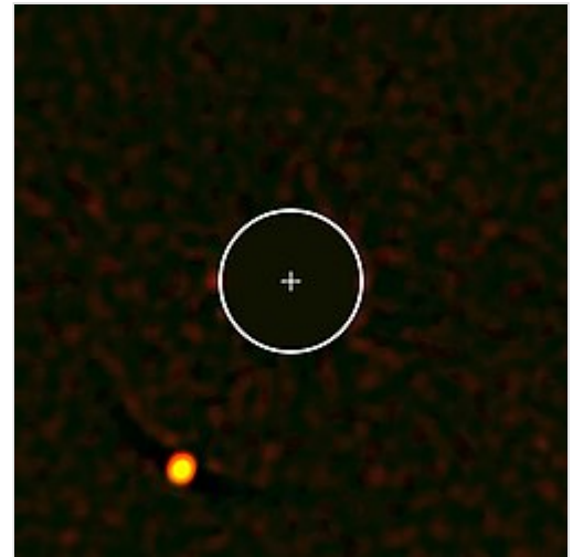
Exoplanet HIP 65426b is the first discovered planet around star HIP 65426 . [42]
