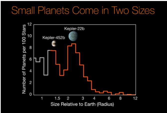
Small planets come in two sizes
