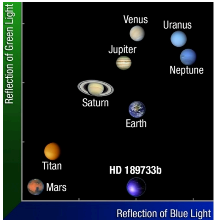
This color-color diagram compares the colors of planets in the Solar System to exoplanet HD 189733b . The exoplanet's deep blue color is produced by silicate droplets, which scatter blue light in its atmosphere.
