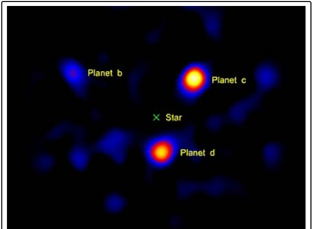
The three known planets of the star HR 8799 , as imaged by the Hale Telescope . The light from the central star was blanked out by a vector vortex coronagraph .
