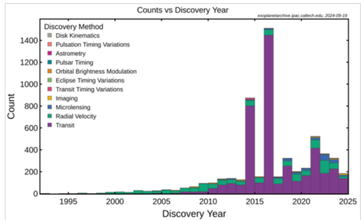
Exoplanet detections per year as of September 2024 [48]
