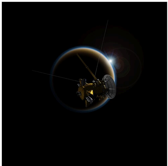
Sunset studies on Titan by Cassini help understand exoplanet atmospheres (artist's concept).
