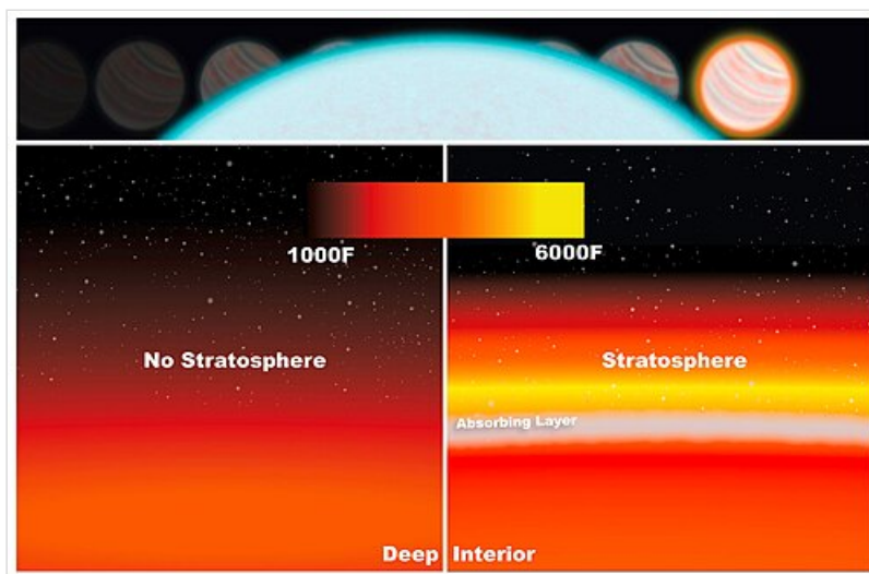
Artist's illustration of temperature inversion in exoplanet's atmosphere. [194]
