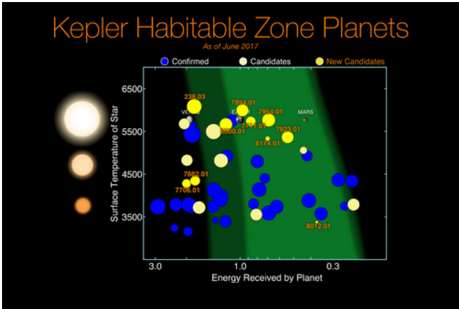
Kepler habitable zone planets
