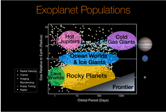
Exoplanet populations; colors indicate detection method
