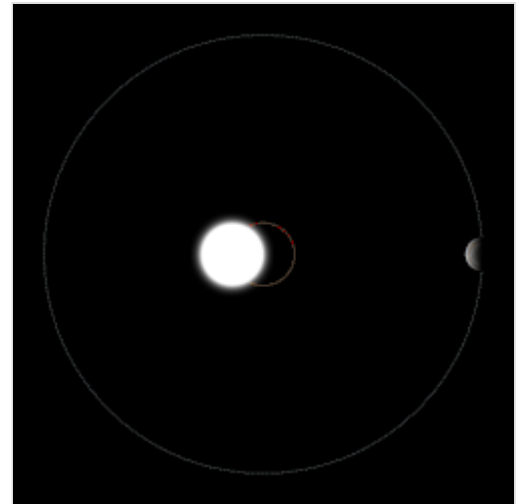
A planet is able to gravitationally pull its host star 🔍
