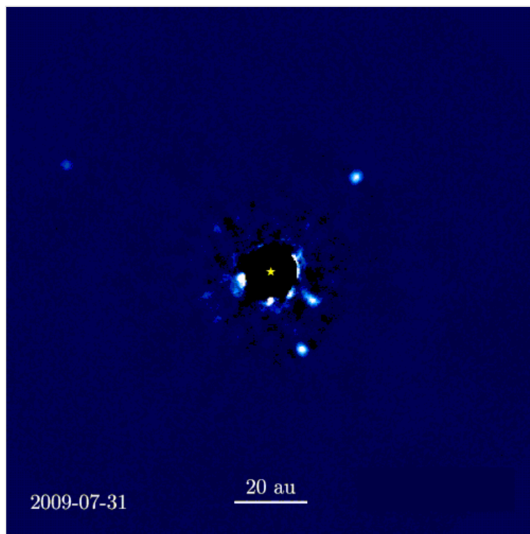
Four exoplanets of the HR 8799 system imaged by the W. M. Keck Observatory over the course of seven years. Motion is interpolated from annual observations. ↗
