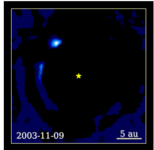
Directly imaged planet Beta Pictoris b , with an edge-on orbit as seen from Earth
