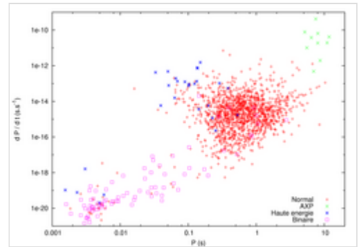
P – P -dot diagram for known rotation-powered pulsars (red), anomalous X-ray pulsars (green), high-energy emission pulsars (blue) and binary pulsars (pink)
