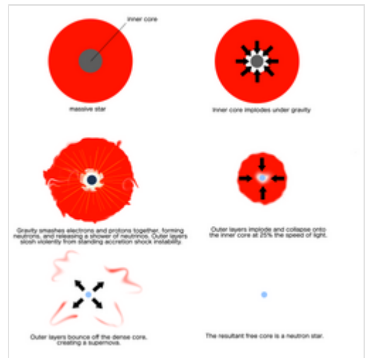
Simplified representation of the formation of neutron stars
