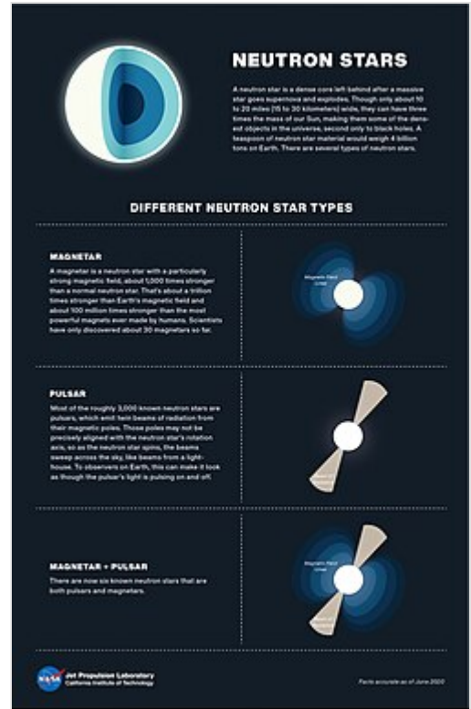
Different types of neutron stars
