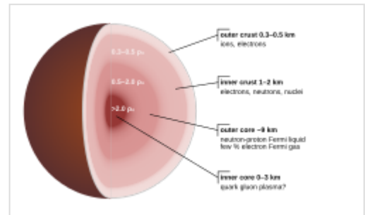
Cross-section of neutron star. Densities are in terms of \rho_0 the saturation nuclear matter density, where nucleons begin to touch.
