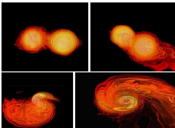
Four snapshots from a computer simulation of a neutron star merger. From top left:
