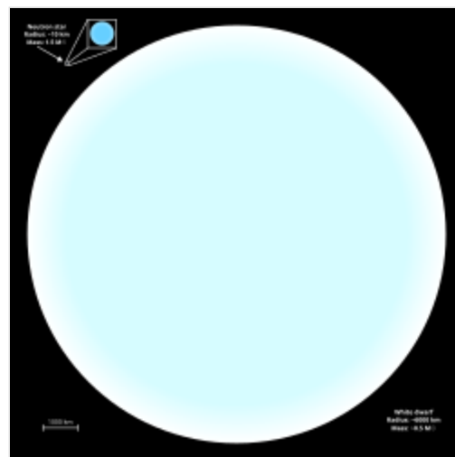
Comparison of a 10-km-radius neutron star (top left corner) and a 6,000-km-radius white dwarf , the latter roughly the size of Earth
