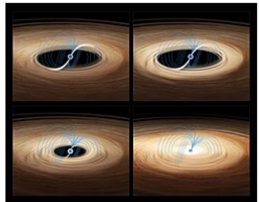
Computer renders of a neutron star with accretion disk , with magnetic field lines projected, showing bursts of powerful X-rays . The simulations are taken from 2017 data from NASA's NuSTAR and Swift, and ESA's XMM-Newton observatories.
