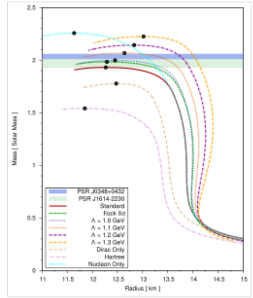
Neutron star mass–radius relationships for several scenarios. Black dots indicate highest-mass stars, and colored bars represent constraints by observed pulsars.
