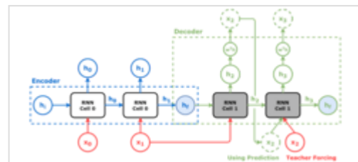
Encoder-decoder RNN without attention mechanism. Teacher forcing is shown in red. □
