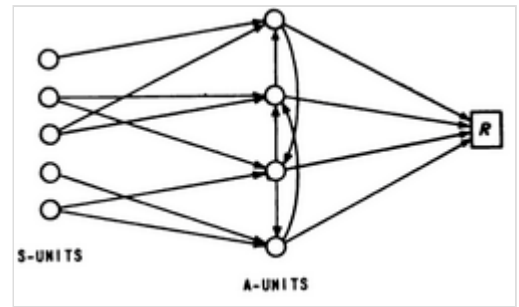
A close-loop cross-coupled perceptron network [17]:403, Fig. 47
