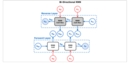
Bidirectional RNN
