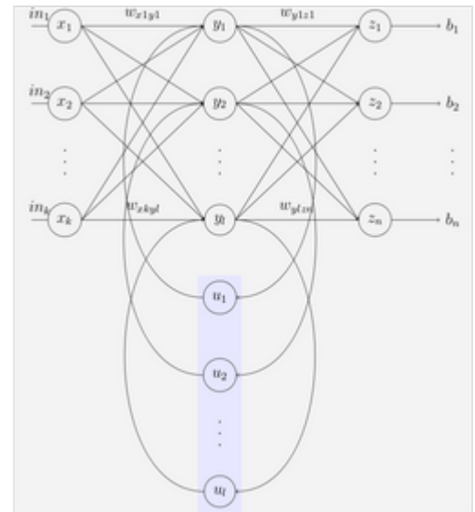
The Elman network
