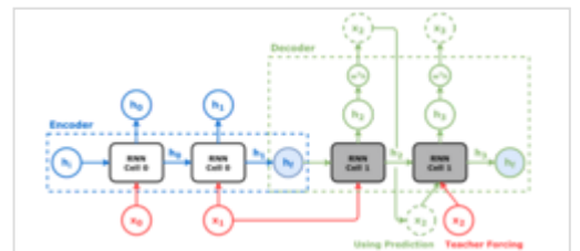
Encoder-decoder RNN without attention mechanism
