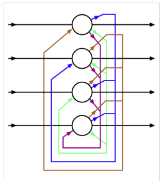
A fully connected RNN with 4 neurons
