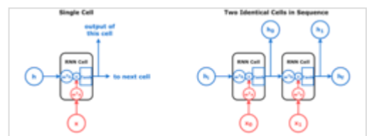
A simple Elman network where \sigma_h = \tanh, \sigma_y = \text{Identity}
