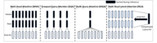
Comparison between several different forms of attention mechanism and the amount of KV caching necessary for each
