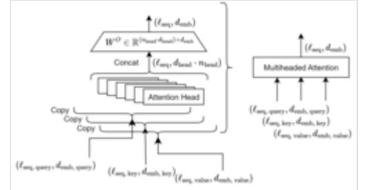
Exact dimension counts within a multihead attention module
