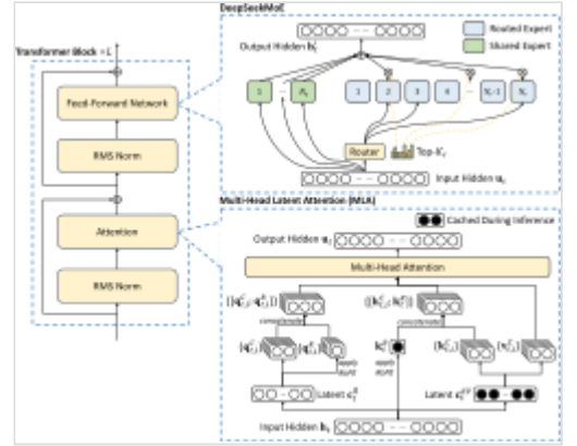
The architecture of V2, showing both MLA and a variant of mixture of experts [90] : Figure 2
