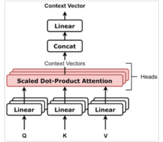
Multihead attention, block diagram
