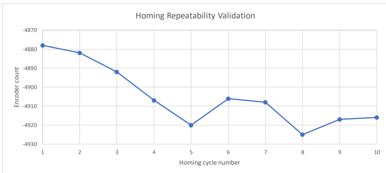
Figure 22 Detected reference position during ten consecutive homing cycles.
