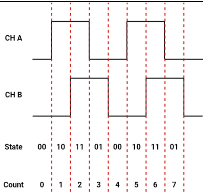
Figure 17 Quadrature encoder state transitions during positive motion
