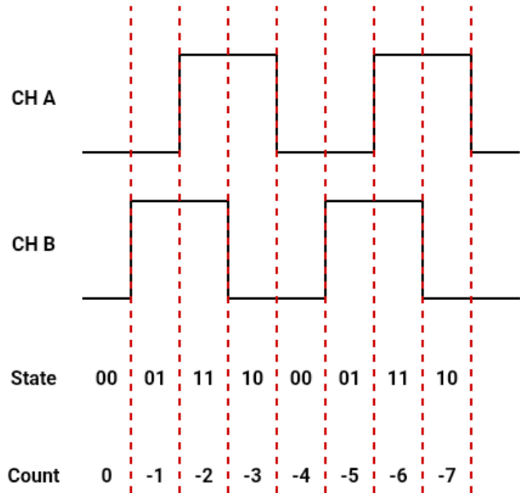
Figure 18 Quadrature encoder state transitions during negative motion
