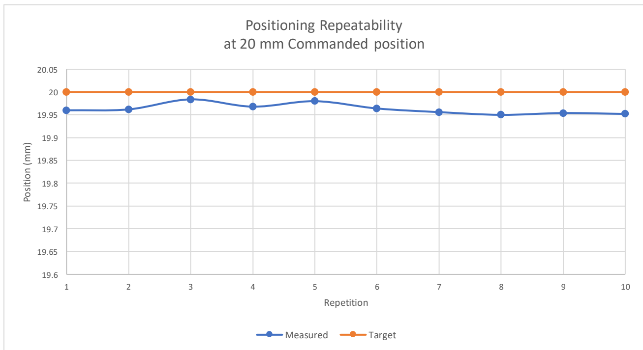
Figure 25 Reported position during ten consecutive commands of 20 mm.
