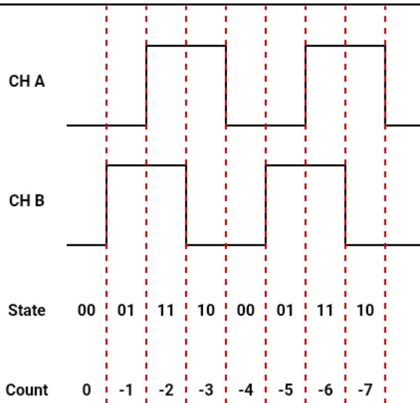
Figure 18 Quadrature encoder state transitions during negative motion
