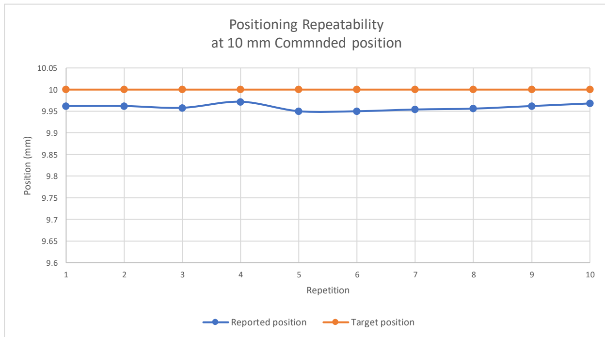
Figure 23 Reported position during ten consecutive commands of 10 mm.
