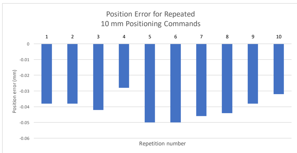
Figure 24 Positioning error observed during ten consecutive commands of 10 mm.
