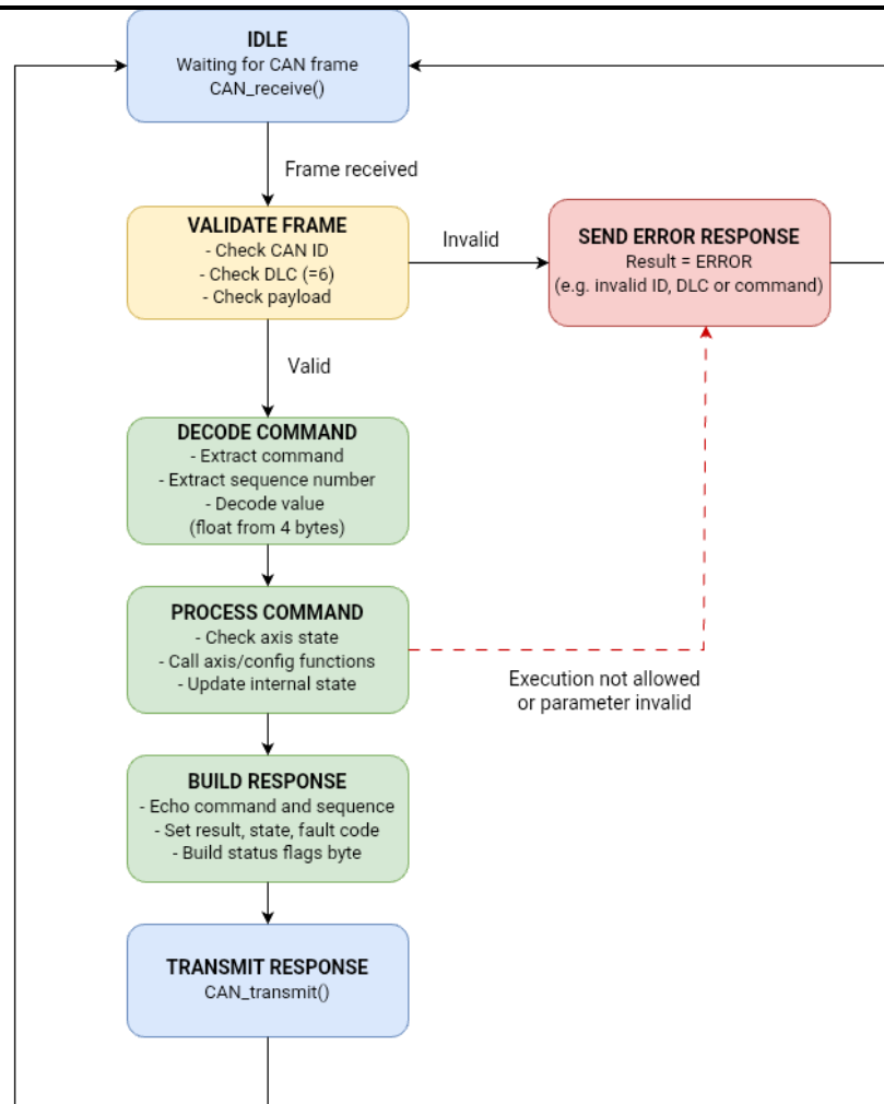
Figure 19 CAN command processing state machine
