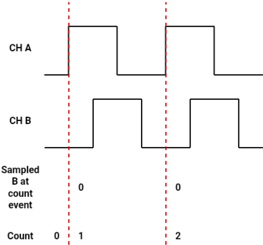
Figure 15 Single-channel encoder counting using channel A rising edges during positive motion
