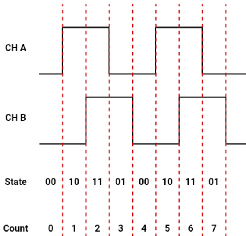
Figure 17 Quadrature encoder state transitions during positive motion
