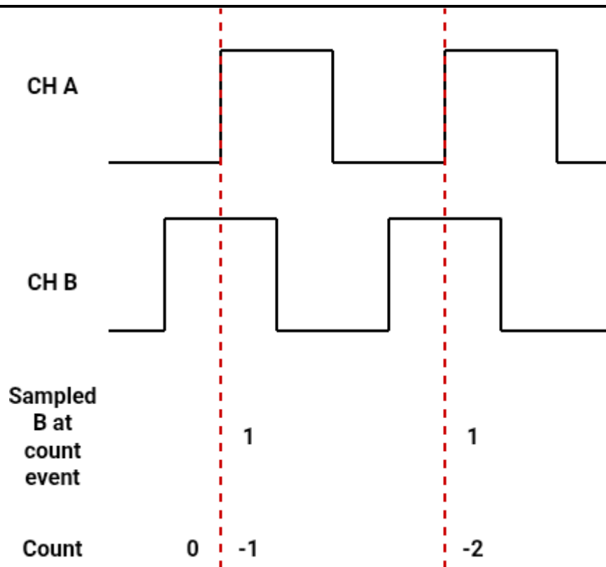
Figure 16 Single-channel encoder counting using channel A rising edges during negative motion
