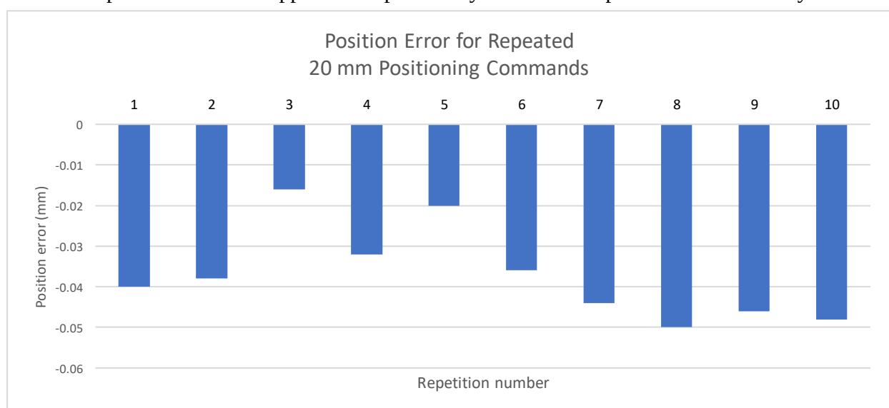
Figure 26 Positioning error observed during ten consecutive commands of 20 mm.
