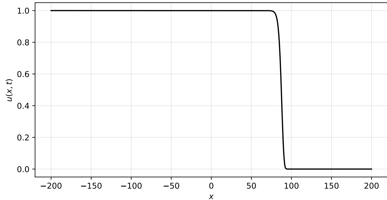
Final invader profile, \gamma = 50.0 , V_\infty = 0.3
