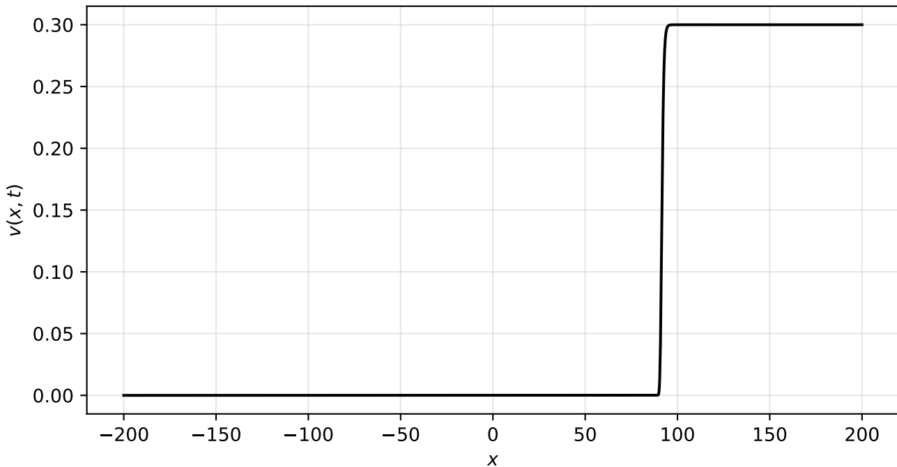
Final resident profile, \gamma = 50.0 , V_\infty = 0.3
