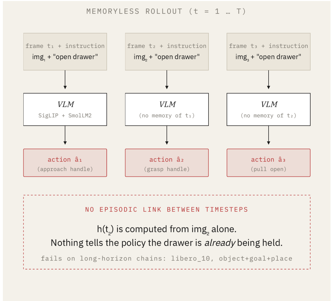
Figure 1: Three timesteps of a memoryless VLA rollout. Each frame is processed independently; there is no episodic link between timesteps. h_t is computed from \text{img}_t alone, so the policy cannot tell that the drawer is already being held.
