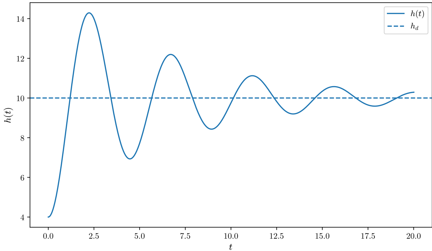
Case 3: No velocity feedback
