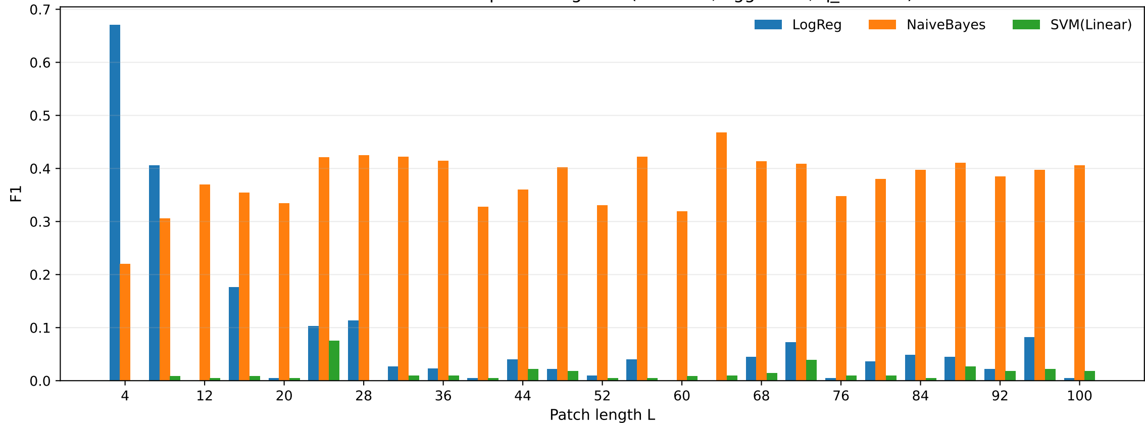
FordB: F1 for different patch lengths L (stride=L, agg=max, q_thr=0.8)
