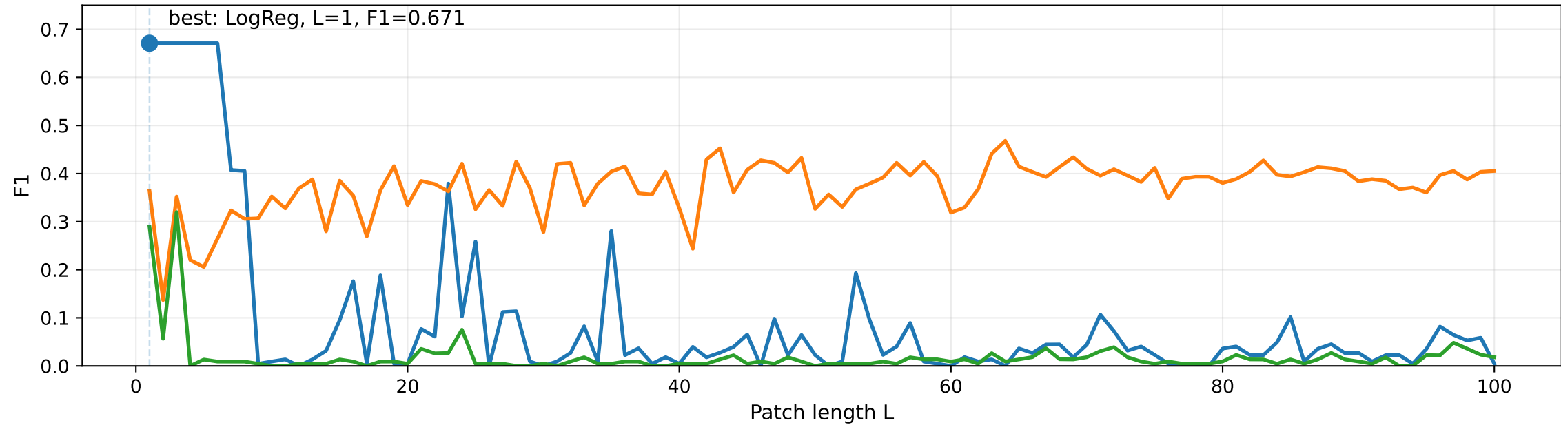
LogReg NaiveBayes SVM(Linear) FordB: F1 vs patch length L (agg=max, q_thr=0.8)
