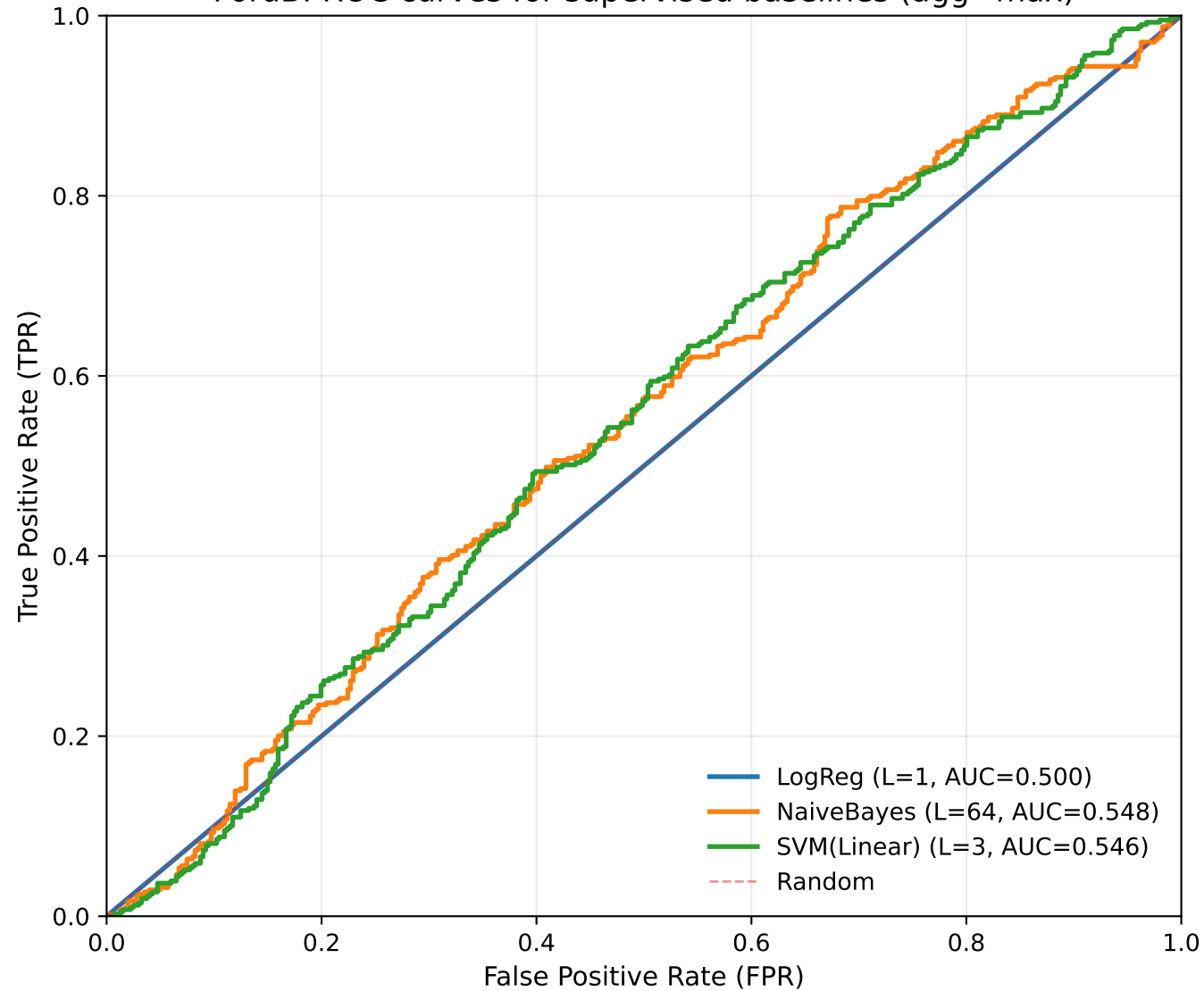
FordB: ROC curves for supervised baselines (agg=max)
