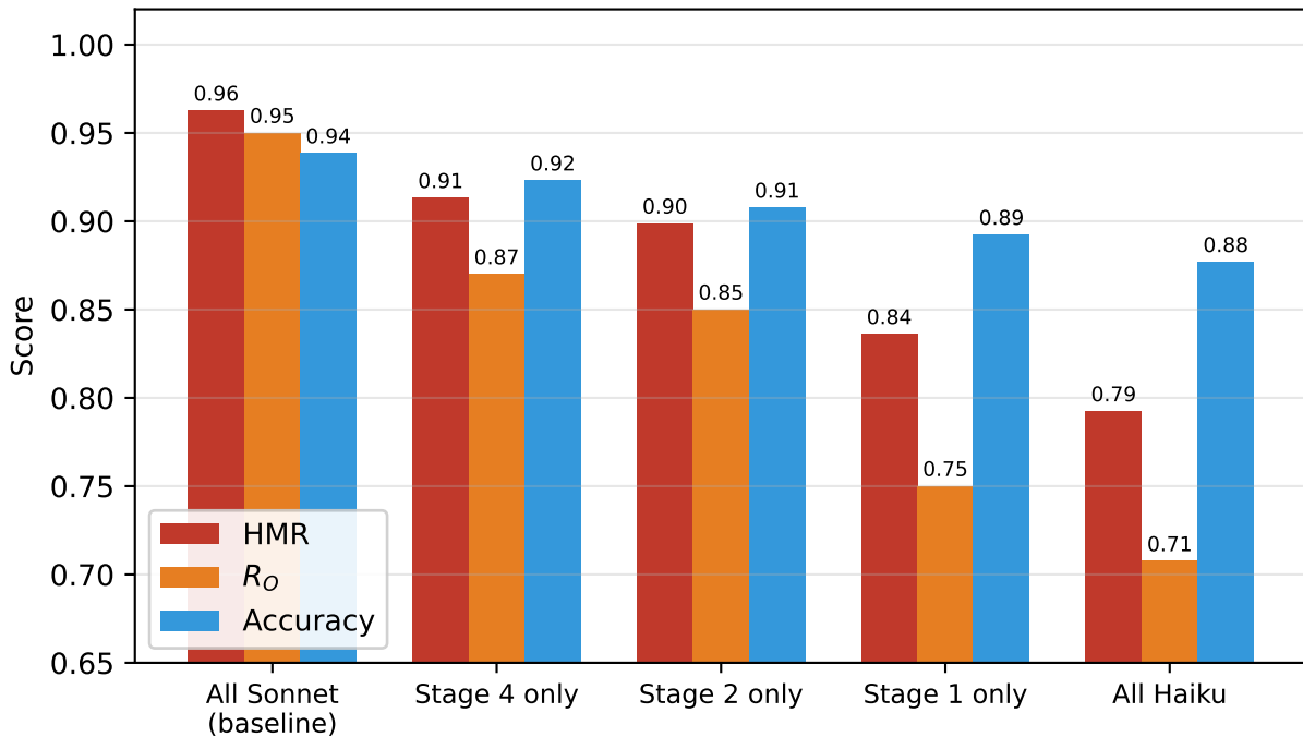
RQ10: Per-stage Sonnet→Haiku ablation. Stage 1 is most critical.
