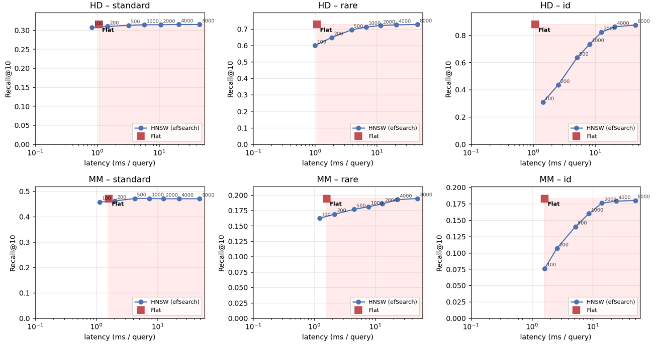
Fig. 4. Recall@10 vs. per-query latency. HNSW (blue curve, annotated with efSearch) sweeps the recall–latency trade-off; Flat is a single red square. Red shading marks the region Pareto-dominated by Flat (slower and lower recall). On standard subsets HNSW efS= 100 sits inside the frontier (slightly faster than Flat at \geq 97\% recall): the canonical ANN sweet spot. On ID subsets, the entire HNSW curve lies in the dominated region until efS \geq 4000 , where HNSW is \sim 8\text{--}19\times slower than Flat to match its recall.
