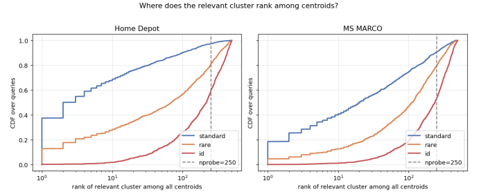
Fig. 4. CDF of the rank, among all 500 centroids, of each query’s relevant cluster. Dashed line marks n_{\text{probes}}=250 (probe-ratio 0.5); queries to the right of it are guaranteed misses for IVF regardless of in-cluster retrieval quality. For ID queries, 41–47% of relevant clusters fall outside the top-half by centroid score.
