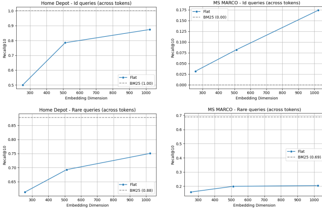
Fig. 5. Flat Recall@10 vs. embedding dimension d for ID (top) and rare (bottom) queries, on Home Depot (left) and MS MARCO (right). BM25 shown as dashed reference.
