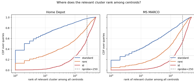
Fig. 4. CDF of the rank, among all 500 centroids, of each query’s relevant cluster. Dashed line marks n_{\text{probes}}=250 (probe-ratio 0.5); queries to the right of it are guaranteed misses for IVF regardless of in-cluster retrieval quality. For ID queries, 41–47% of relevant clusters fall outside the top-half by centroid score.
