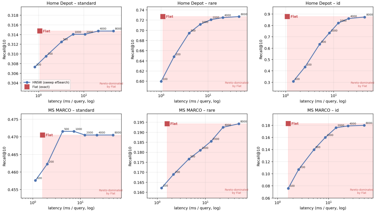
Fig. 4. Recall@10 vs. per-query latency (log-x), single-threaded with warm-up. HNSW sweeps efSearch \in \{100, \dots, 8000\} (blue curve, annotated); Flat is one red square. Red shading marks the region strictly dominated by Flat (slower and lower recall). Across all subsets, Flat upper-bounds recall by construction; the question is how much efSearch budget HNSW needs to approach it. On standard subsets a few hundred suffice. On ID subsets the HNSW curve climbs slowly and approaches Flat’s recall only at efS \geq 2000 –4000.
