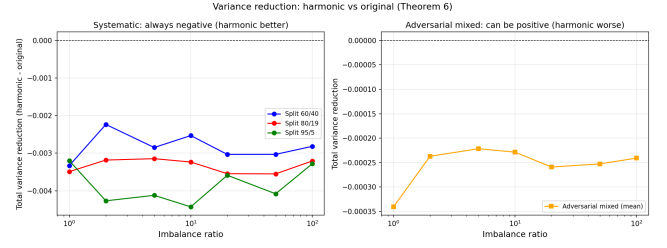
Figure 6: Variance reduction achieved by harmonic vs. original across systematic and adversarial mixed-imbalance configurations. Harmonic reduces total variance in 100% of systematic cases (Cauchy–Schwarz guarantee), and the D_k \geq 0 sufficient condition holds in 46.6% of those cases.
