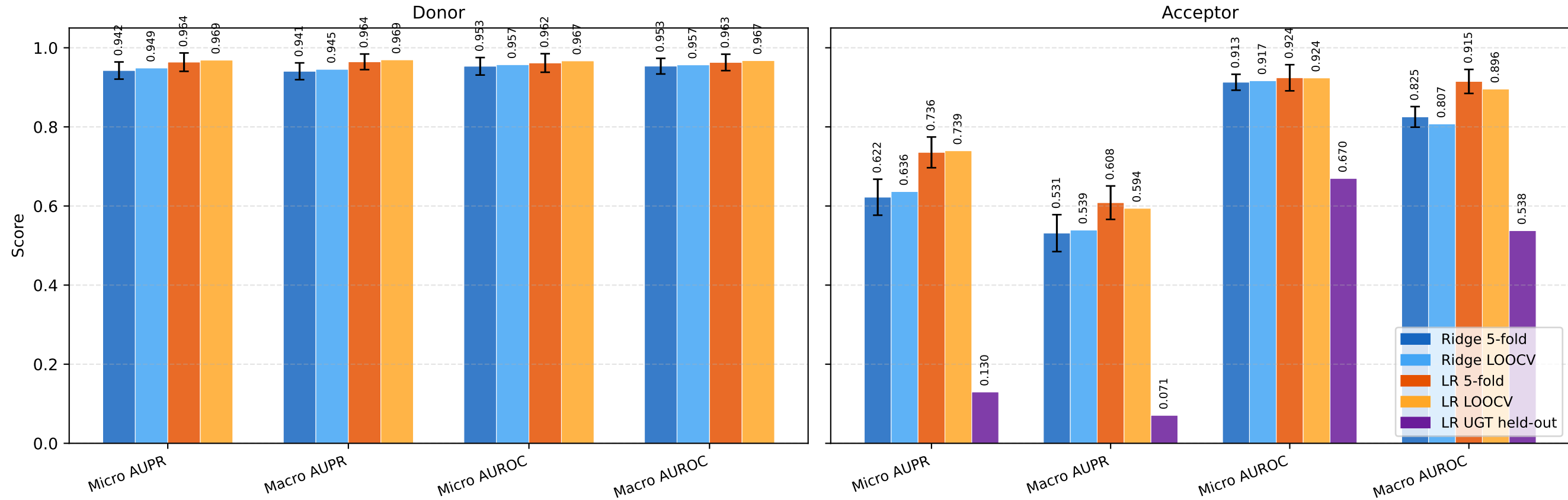
Figure 5 — Ridge (FL) vs LR (LL): BAHD CV and UGT Held-Out
