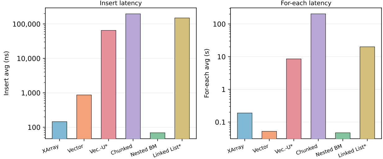
Figure 9: Insert latency (left) and for-each latency (right) per backend on a log scale. Both axes span multiple orders of magnitude; backends marked * were measured at 512 MB.
