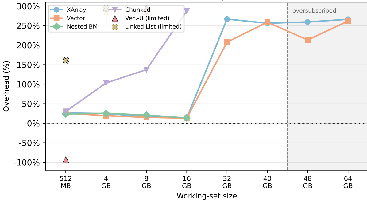
GEMM overhead by backend
