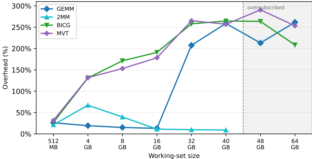
Overhead: Polybench kernels (GEMM, 2MM, BICG, MVT)
