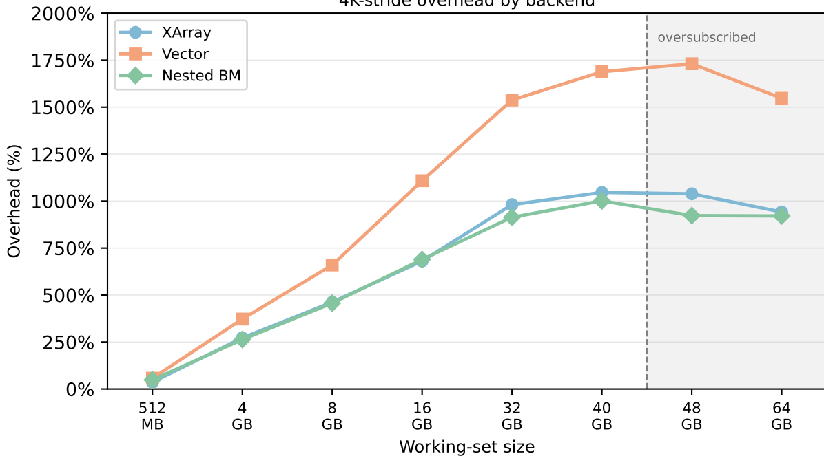
4K-stride overhead by backend
