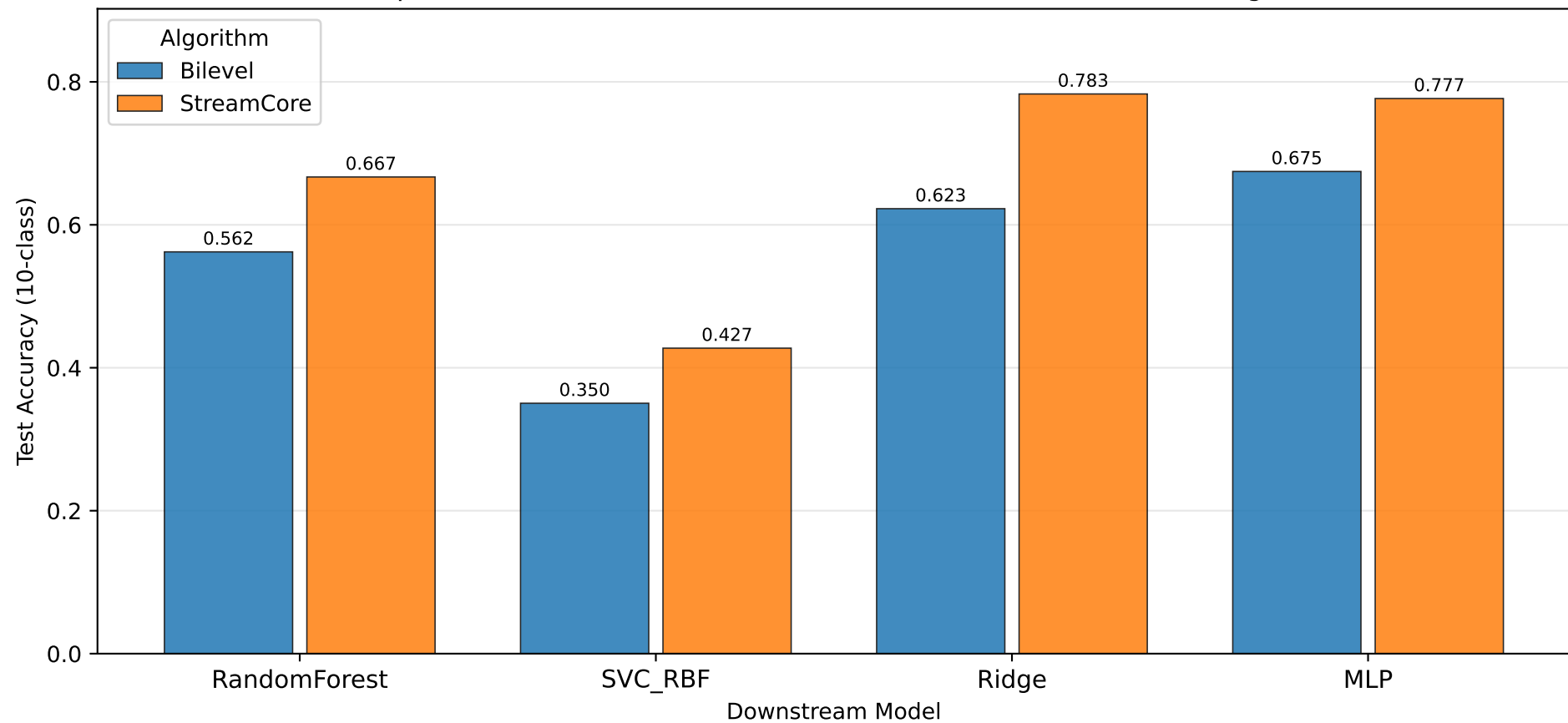
Split-MNIST: StreamCore vs Bilevel (M=50, ResNet-18 embeddings)
