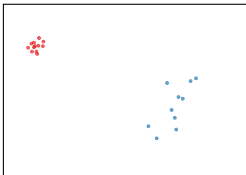
Proposed (Weighted)
