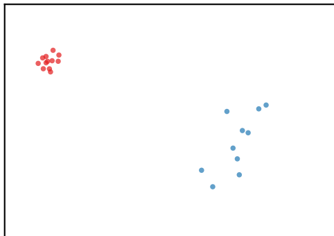
Unweighted (Naive)
