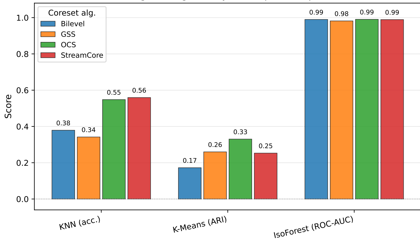
Task agnostic (geometry & unsupervised probes)
