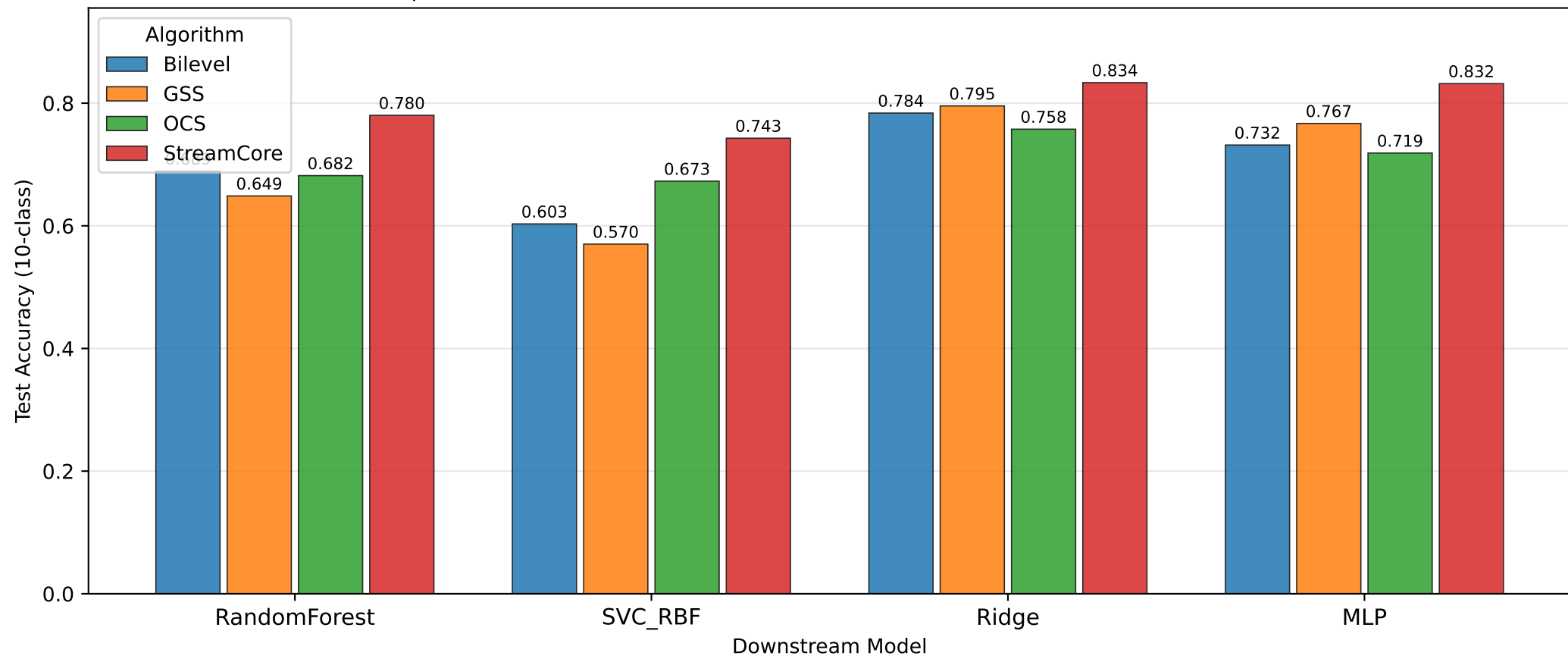
Split-MNIST: StreamCore vs Bilevel vs OCS vs GSS (M=100, ResNet-18)
