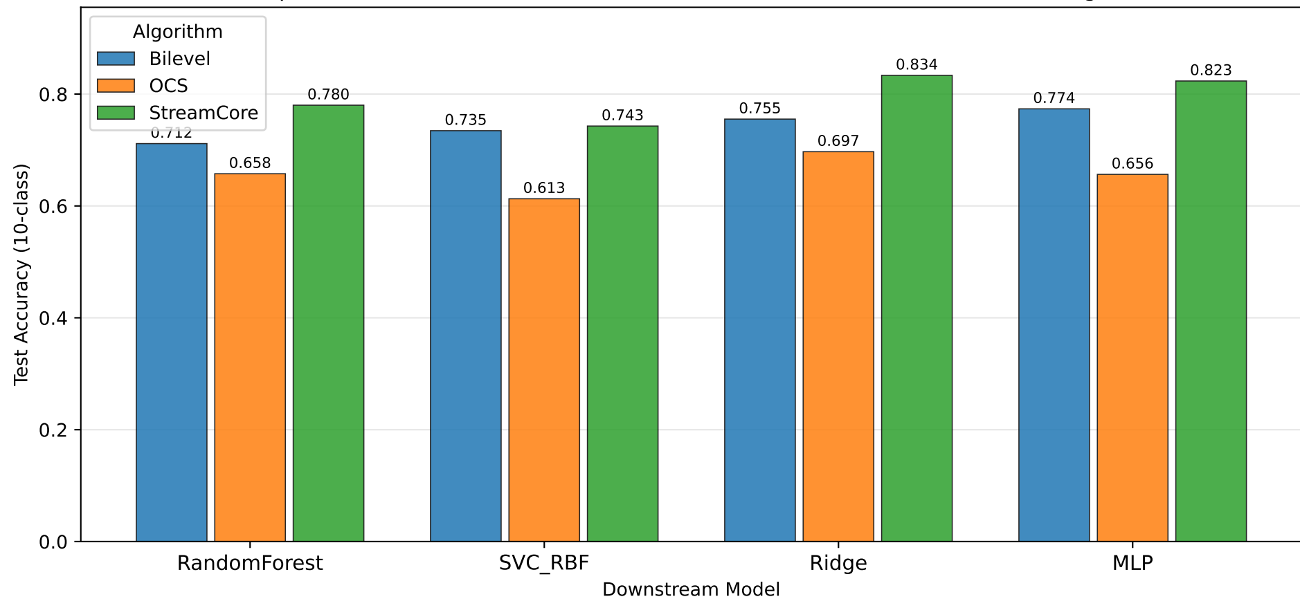
Split-MNIST: StreamCore vs Bilevel vs OCS (M=100, ResNet-18 embeddings)
