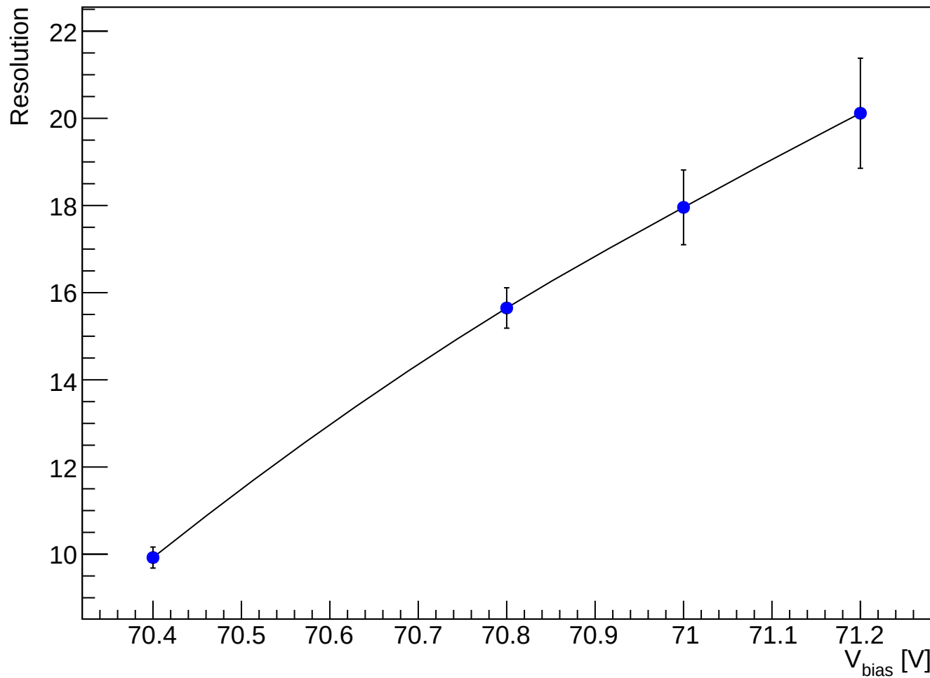
Resolution Vs V_{\text{bias}}
