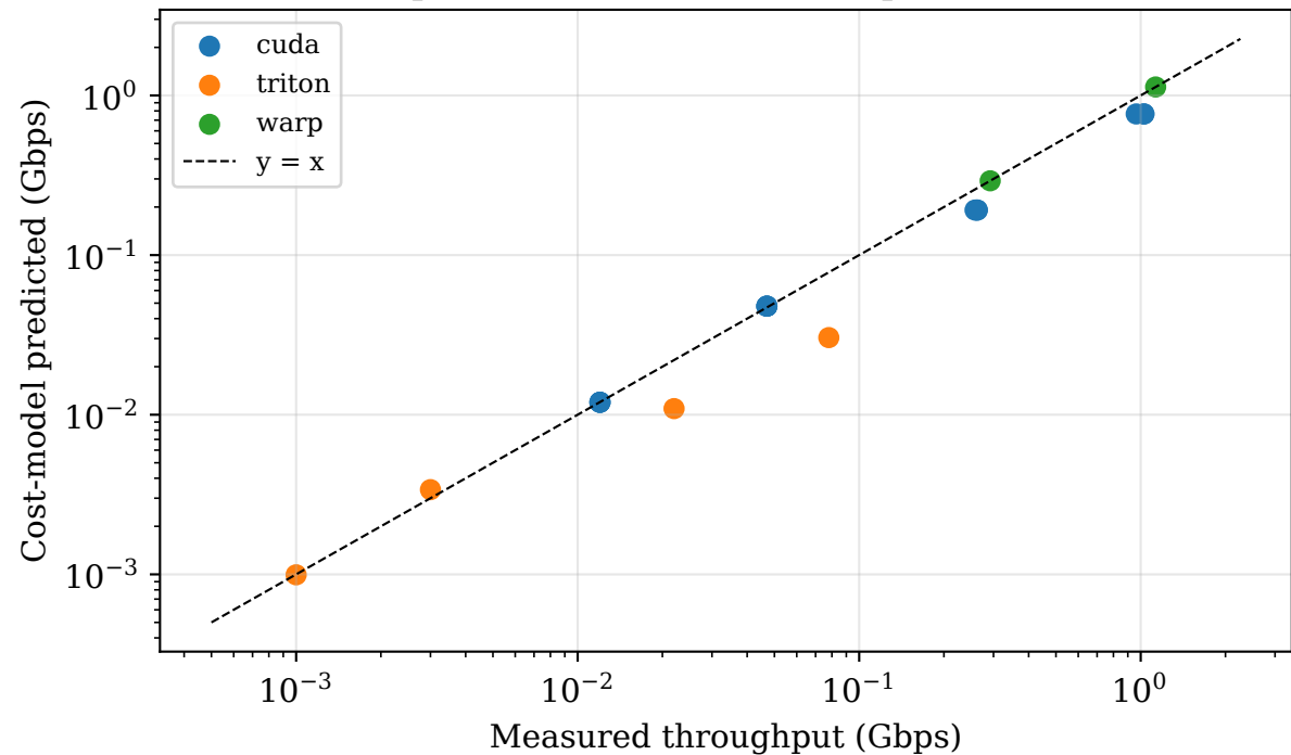
Cost model: predicted vs measured (per-backend n^2 fit)
