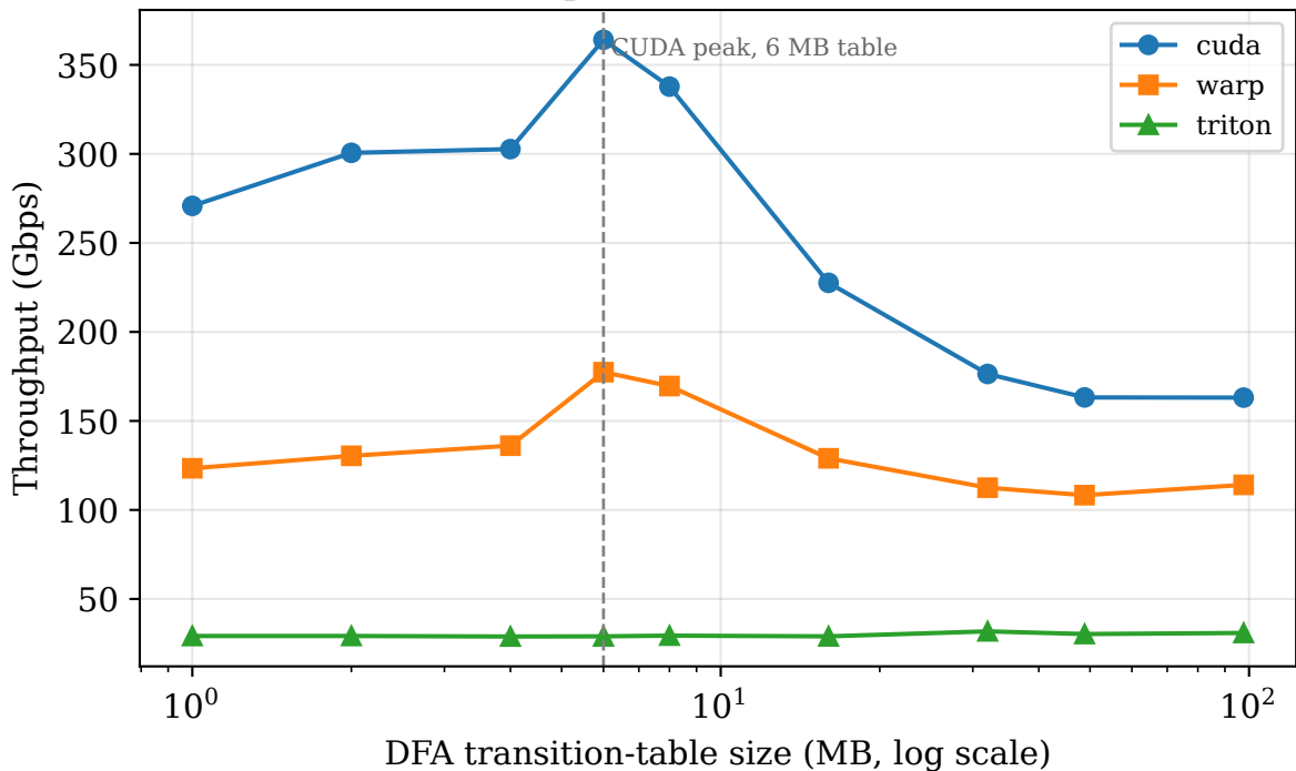
DFA face: CUDA and Warp rise then fall with table size; Triton flat
