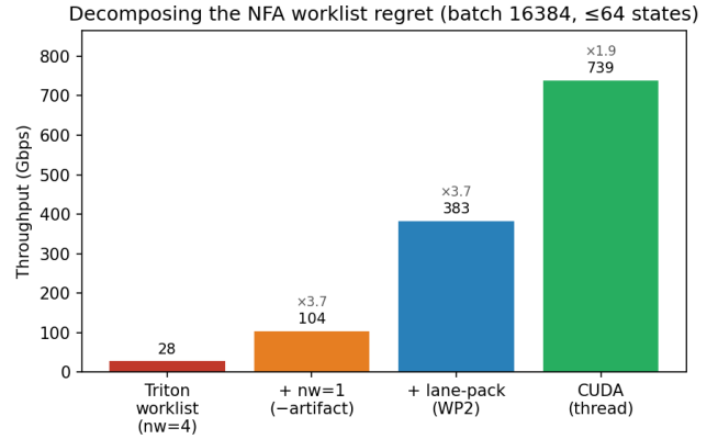
Figure 1. NFA worklist throughput (batch 16384, \leq 64 states) climbs as each regret component is removed: nw=4 \rightarrow nw=1 (launch artifact), \rightarrow lane-packing (warp redundancy), \rightarrow CUDA (irreducible latency). All oracle-gated.
