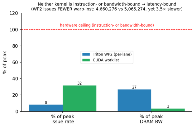
Figure 4. Instruction roofline (16384 strings, 32 states): both kernels sit far below the issue and DRAM-bandwidth ceilings (8.3%/27% for Triton, 32%/3.4% for CUDA), so neither is instruction- nor bandwidth-bound: the residual is latency.
