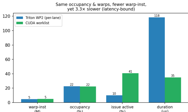
Figure 3. Per-lane Triton vs. CUDA (16384 strings, 32 states): same occupancy, fewer warp-instructions, yet 3.3\times slower at 9.9% vs. 41% issue activity: latency-bound.
