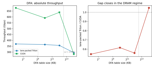
Figure 5: DFA: lane-packed Triton trails CUDA \sim 1.7\times while the table is cache-resident but matches it ( 1.05\times ) once the 16 MB table spills past L2—both then rely on cross-warp parallelism. The residual is regime-dependent.
