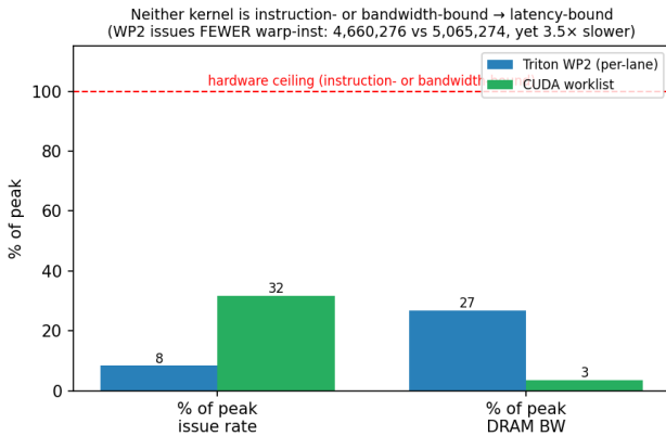
Figure 4: Instruction roofline (16384 strings, 32 states): both kernels sit far below the issue and DRAM-bandwidth ceilings (8.3%/27% for Triton, 32%/3.4% for CUDA), so neither is instruction- nor bandwidth-bound—the residual is latency.
