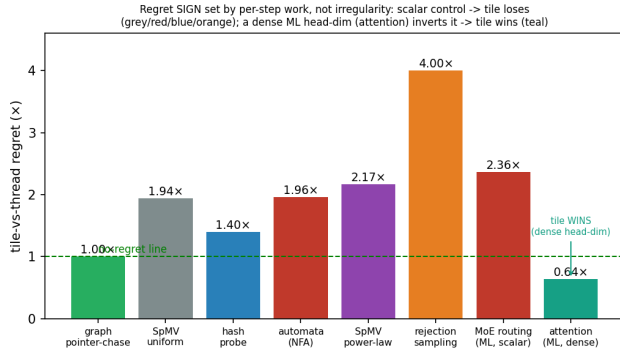
Figure 7: The regret law across eight oracle-gated irregular workloads, by dominant mechanism. A graph pointer-chase (green) is the negative control (irregular memory + dependent loads, no control divergence \Rightarrow regret 1.00 \times ). Regret grows with scalar control / divergence (grey, red, blue, orange), peaking at 4 \times . The two ML witnesses (right) test the sign : MoE routing (scalar per step) confirms the law (2.36 \times ), while ragged attention (dense head-dim) inverts it (0.64 \times , teal, below the no-regret line—the tile wins), because per-step instruction efficiency, not irregularity, sets the sign.
