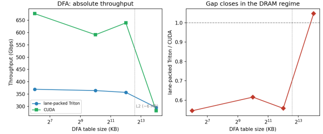
Figure 5: DFA: lane-packed Triton trails CUDA \sim 1.7\times while the table is cache-resident but matches it ( 1.05\times ) once the 16 MB table spills past L2—both then rely on cross-warp parallelism. The residual is regime-dependent.
