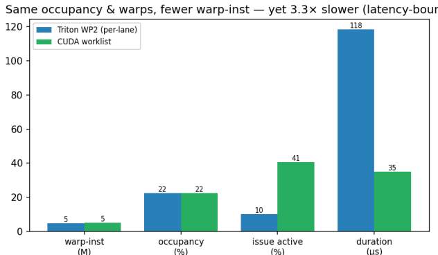
Figure 3: Per-lane Triton vs. CUDA (16384 strings, 32 states): same occupancy, fewer warp-instructions, yet 3.3× slower at 9.9% vs. 41% issue activity—latency-bound.
