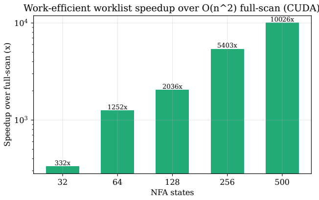
Fig. 3. Work-efficient worklist speedup over O(n^2) full-scan (CUDA), growing with state count.
