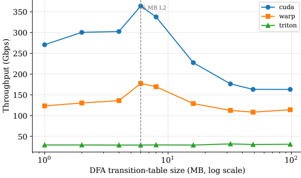
DFA memory-bound face: CUDA/Warp peak at L2 then drop; Triton flat
