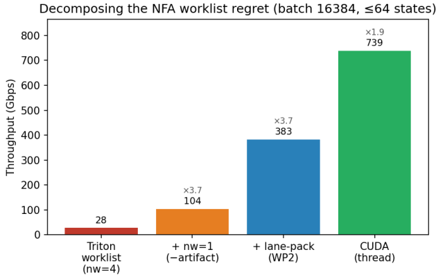
Figure 1. NFA worklist throughput (batch 16384, \leq 64 states) climbs as each regret component is removed: nw=4 \rightarrow nw=1 (launch artifact), \rightarrow lane-packing (warp redundancy), \rightarrow CUDA (irreducible latency). All oracle-gated.
