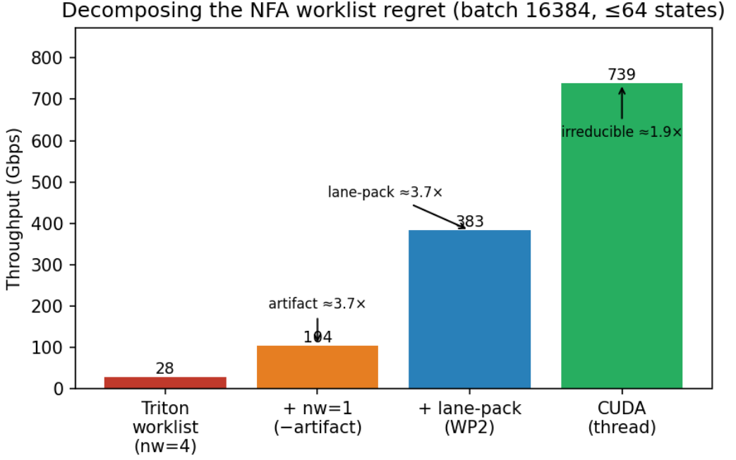
Fig. 1. NFA worklist throughput (batch 16384, \leq 64 states) climbs as each regret component is removed: \text{nw}=4 \rightarrow \text{nw}=1 (launch artifact), \rightarrow lane-packing (warp redundancy), \rightarrow CUDA (irreducible latency). All oracle-gated.
