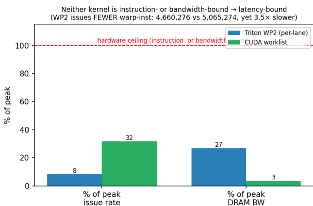
Fig. 4. Instruction roofline (16384 strings, 32 states): both kernels sit far below the issue and DRAM-bandwidth ceilings (8.3%/27% for Triton, 32%/3.4% for CUDA), so neither is instruction- nor bandwidth-bound—the residual is latency.
