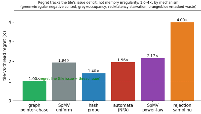
Fig. 7. The regret law across six oracle-gated irregular workloads, by dominant mechanism. A graph pointer-chase (green) is the negative control: irregular memory + dependent loads, no control divergence \Rightarrow tile and thread are identical (issue 5.42% vs. 5.43%) and regret is 1.00x. Regret grows only with scalar control / divergence (red, orange, blue), peaking at 4x for pure control-flow divergence, via two channels (issue starvation, masked-lane waste) over a tile-lowering baseline—scalar control, not memory irregularity.
