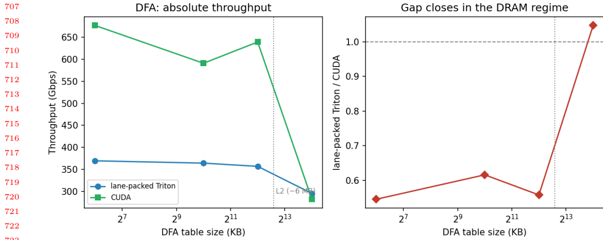
Fig. 5. DFA: lane-packed Triton trails CUDA \sim 1.7\times while the table is cache-resident but matches it ( 1.05\times ) once the 16 MB table spills past L2; both then rely on cross-warp parallelism. The residual is regime-dependent.
