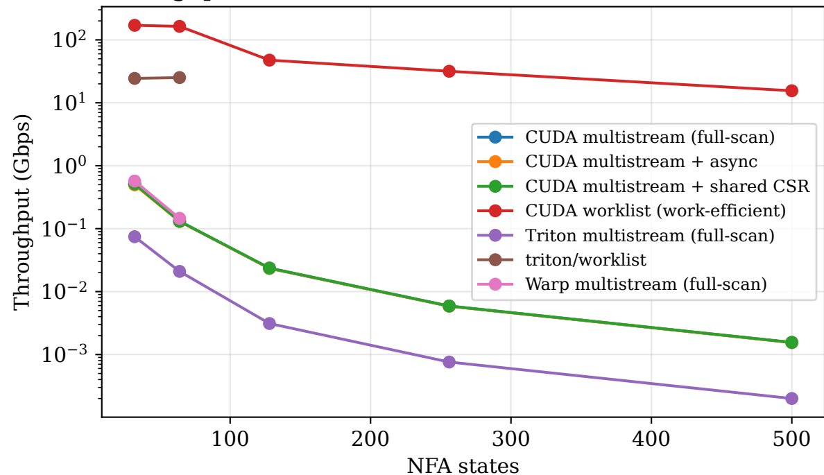
Throughput vs NFA size (batched multi-stream, RTX 4070)
