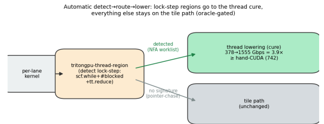
Fig. 8. The automatic detect→route→lower loop (P2). The detection pass (in libtriton) matches the lock-step signature; the lock-step NFA worklist is routed to the thread lowering ( 378\rightarrow 1555 Gbps = 3.9\times , exceeding hand-CUDA), while a no-signature kernel (pointer-chase) stays on the tile path. All routing oracle-gated; numbers from the versioned CSVs.
