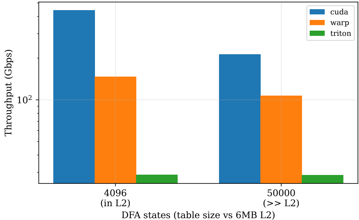
DFA memory-bound face: CUDA/Warp drop past L2; Triton flat (model-bound)
