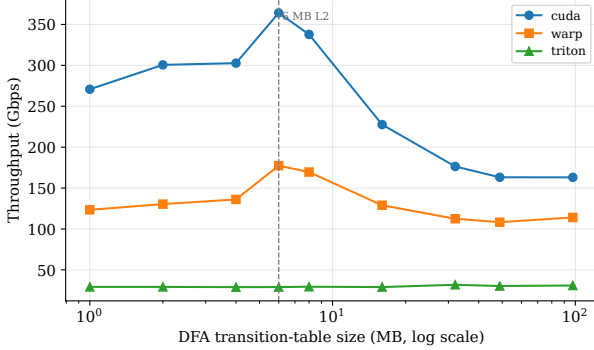
Fig. 6. DFA (memory-bound face), throughput vs table size (log x ), median over 3 random DFAs/size: CUDA/Warp peak at the 6 MB L2 then drop \sim 2.2\times to a DRAM plateau; Triton stays flat (29–32 Gbps)—scalar-gather-bound, never reaching the memory regime.
